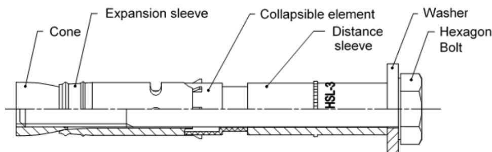
FIGURE 1—COMPONENTS OF THE HSL-3 and HSL-3-R (BOLT VERSION SHOWN)
