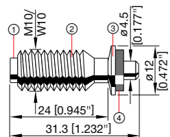
X-BT W10-24-6 SN12-R X-BT M10-24-6 SN12-R
