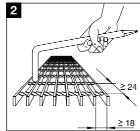
2 Expand grating openings if necessary.
