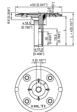
X-FCM-R grating disc
