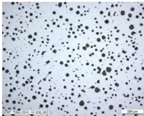
Figure 3. Micro section of cast iron EN-GJS-400-18LT: Spheroidal graphite embedded in ferritic matrix
