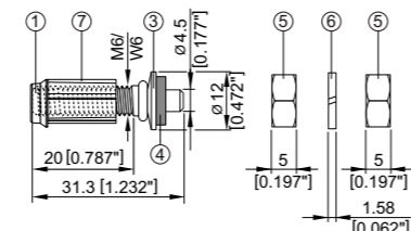
X-BT-ER M6/7 SN 4 X-BT-ER W6/7 SN 4
