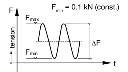
Figure 4. Principle sketch of cyclic tension tests
