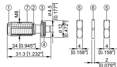
X-BT-ER M8/7 SN 4
