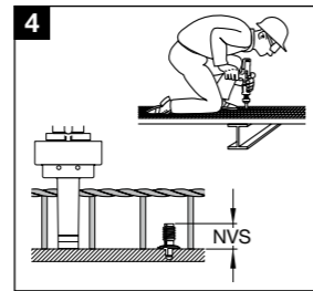
4 Drive fastener only with DX 351 BT G tool and 6.8/11M brown cartridge.
