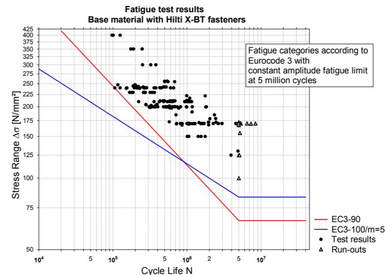
Figure 1. Test data compared with fatigue recommendation according to Eurocode 3 [3]
