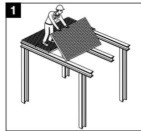
1 Lay grating section in final position.
