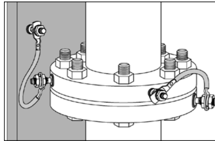
Functional and protective bonding in pipe (Outer diameter of installed surface \geq 150\text{mm} )
