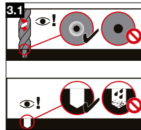
3.1 Pre-drill until shoulder grinds a shiny ring. The drill hole and the area around drilled hole must be clean and free from liquids and debris.
