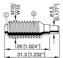
X-BT W10-24-6-R X-BT M10-24-6-R
