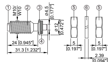
X-BT-ER M10/3 SN 4 X-BT-ER W10/3 SN 4
