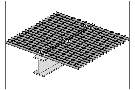
X-FCM-R grating disc
