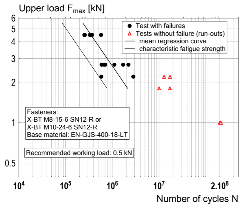
Figure 6. Results of cyclic tension tests
