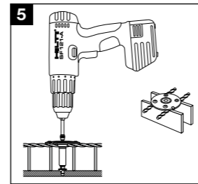
5 Tighten X-FCM-R with 5 mm Allen-type bit.
