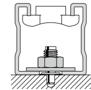
One X-BT stud in each slotted hole
