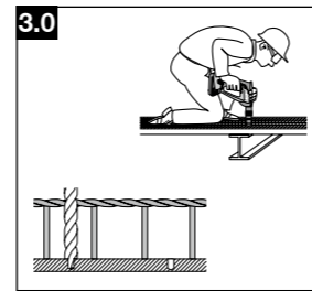
3.0 Pre-drill with TX-BT 4/7 step shank drill bit.
