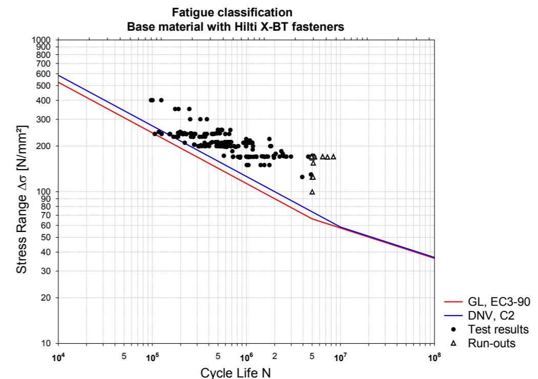
Figure 2. Test data compared with approved GL and DNV fatigue categories
