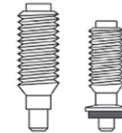
FIGURE 2—HILTI X-BT BLUNT-TIP THREADED STUD WITH AND WITHOUT SN12-R SEALING WASHER
